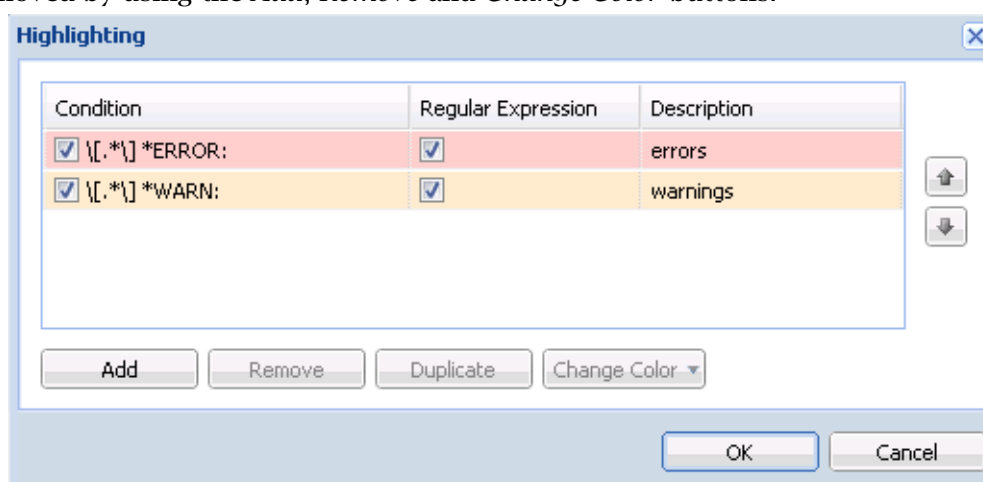
Figure 4.14 Highlighting
