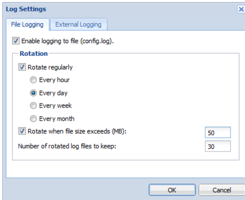
Figure 4.15 File Logging
