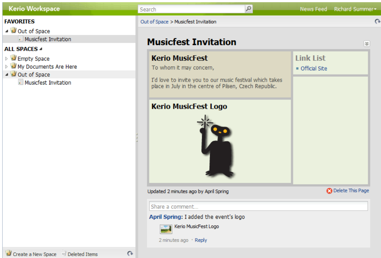
Figure 5.3 User's space
