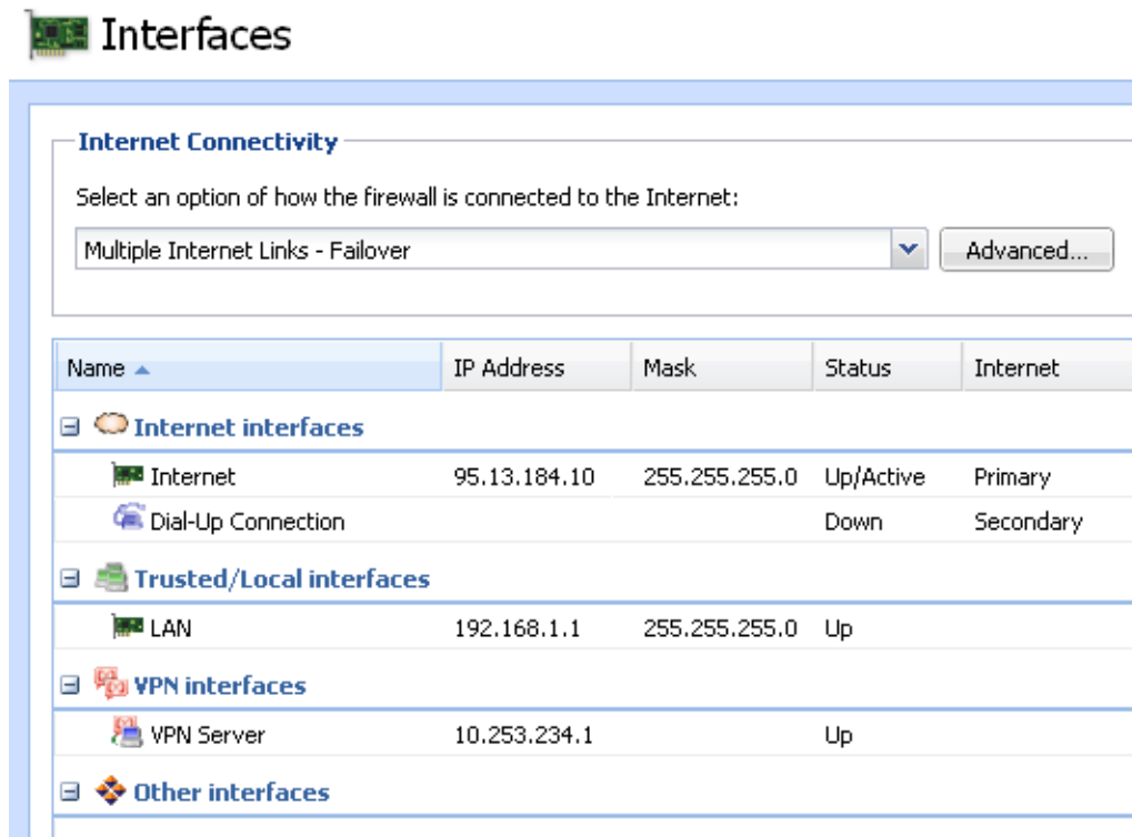
Figure 7.6 Configuration of interfaces — Internet connection failover
