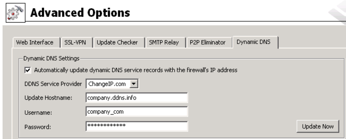
Figure 9.14 Setting cooperation with dynamic DNS server
