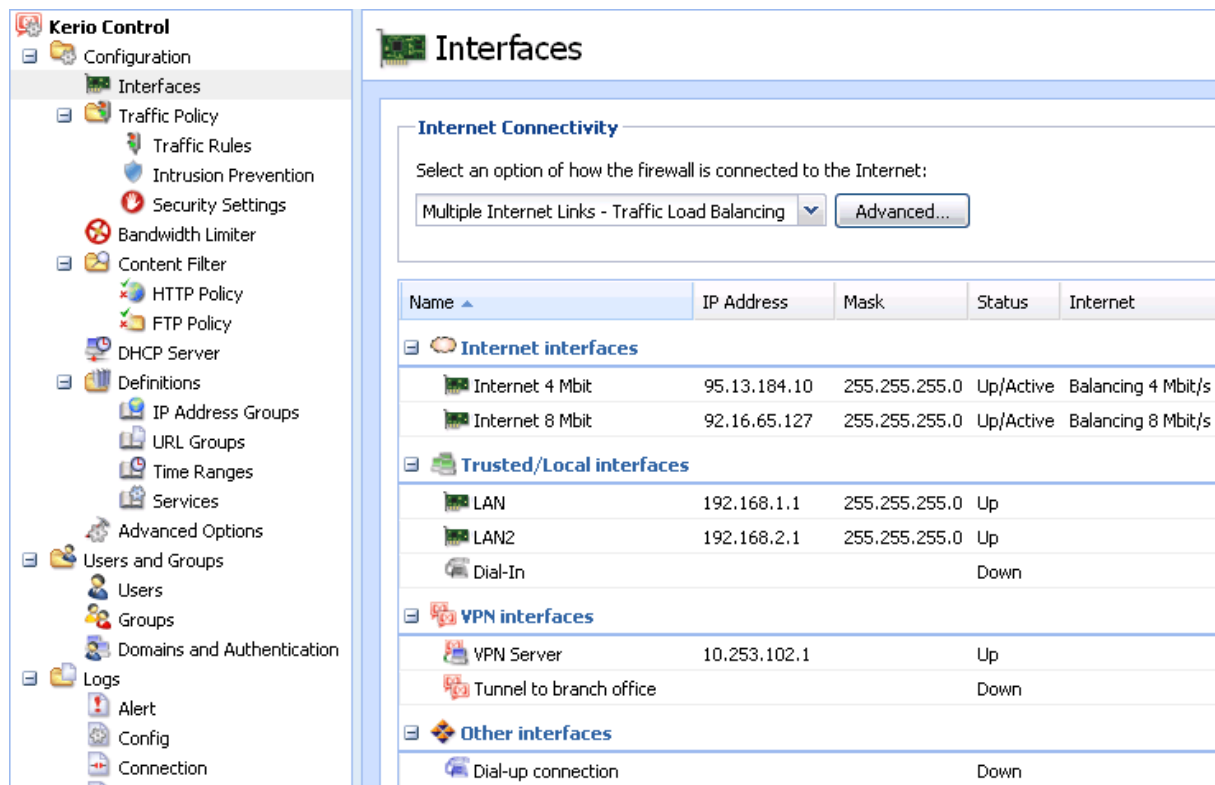
Figure 3.1 Main window of the Kerio Control Administration interface
