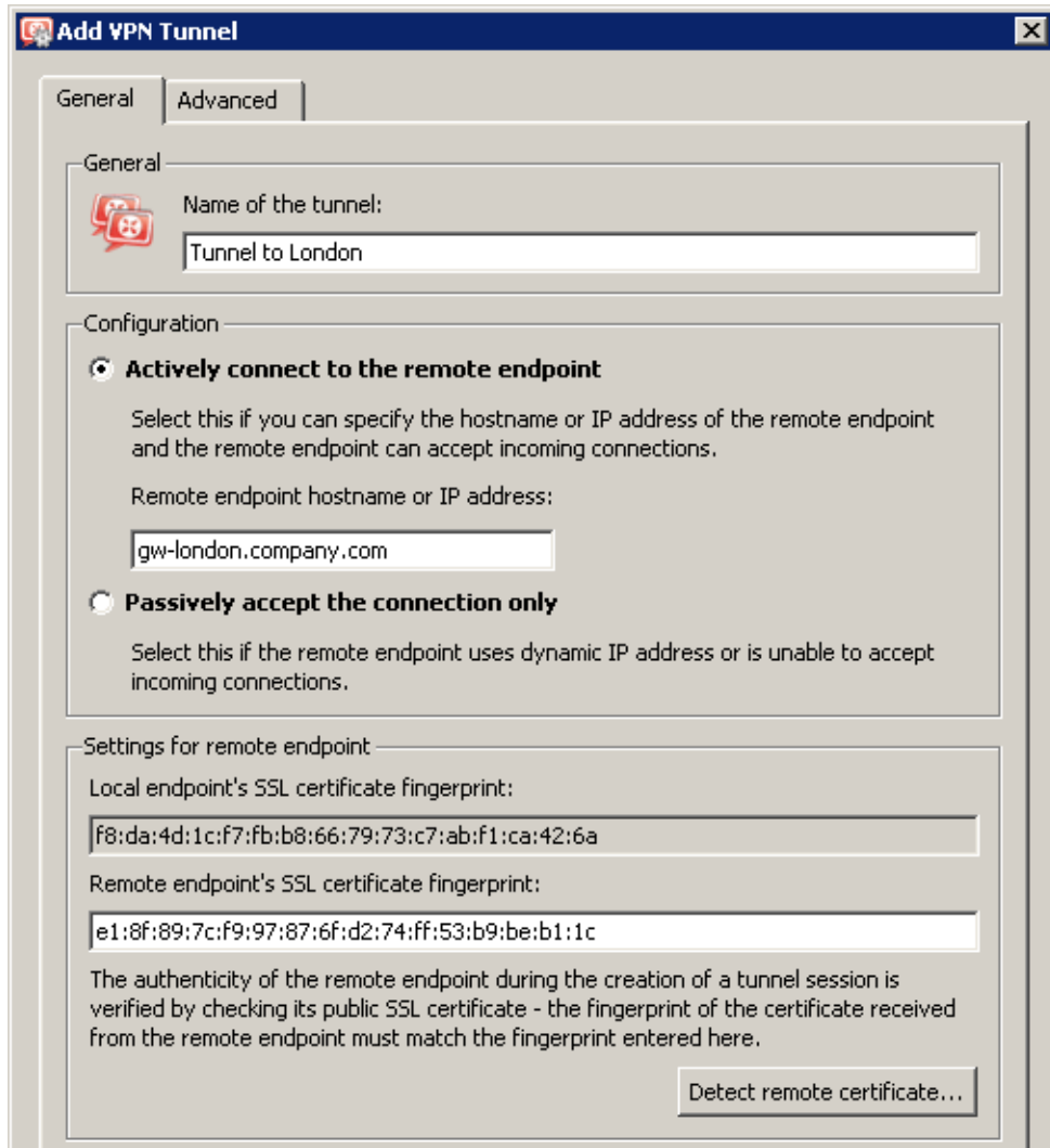
Figure 23.53 The Paris filial office — definition of VPN tunnel for the London filial office
