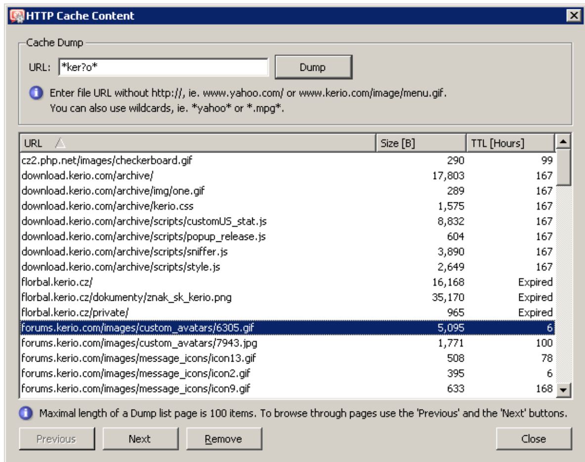
Figure 9.19 HTTP cache administration dialog
