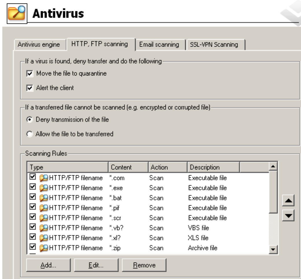
Figure 14.7 Settings for HTTP and FTP scanning
