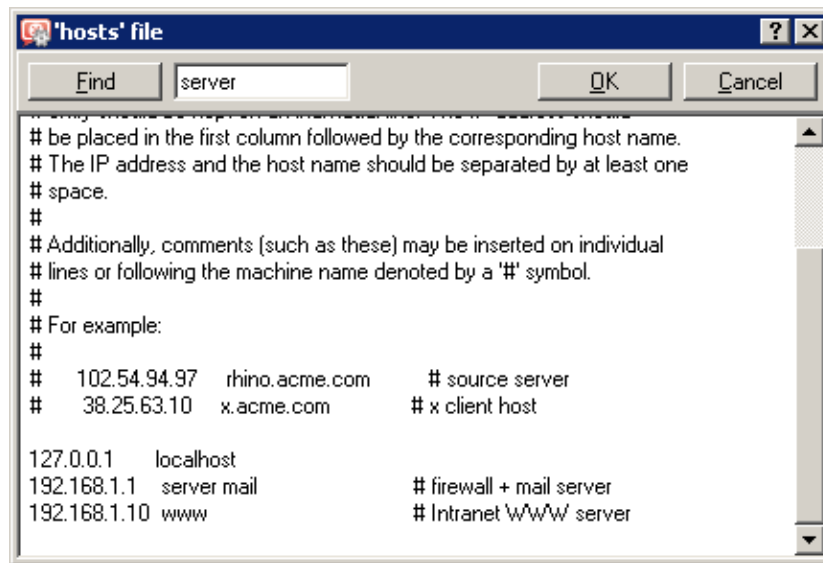
Figure 9.2 Editor of the Hosts system file
