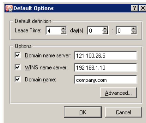
Figure 9.6 DHCP server — default DHCP parameters
