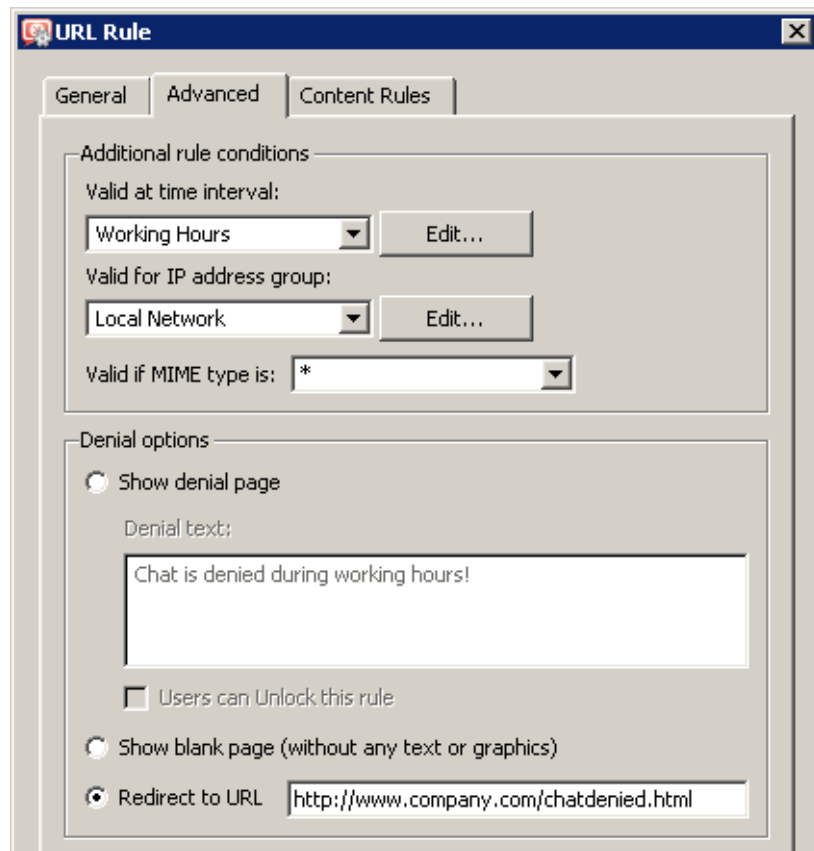
Figure 13.3 URL Rule — advanced parameters
