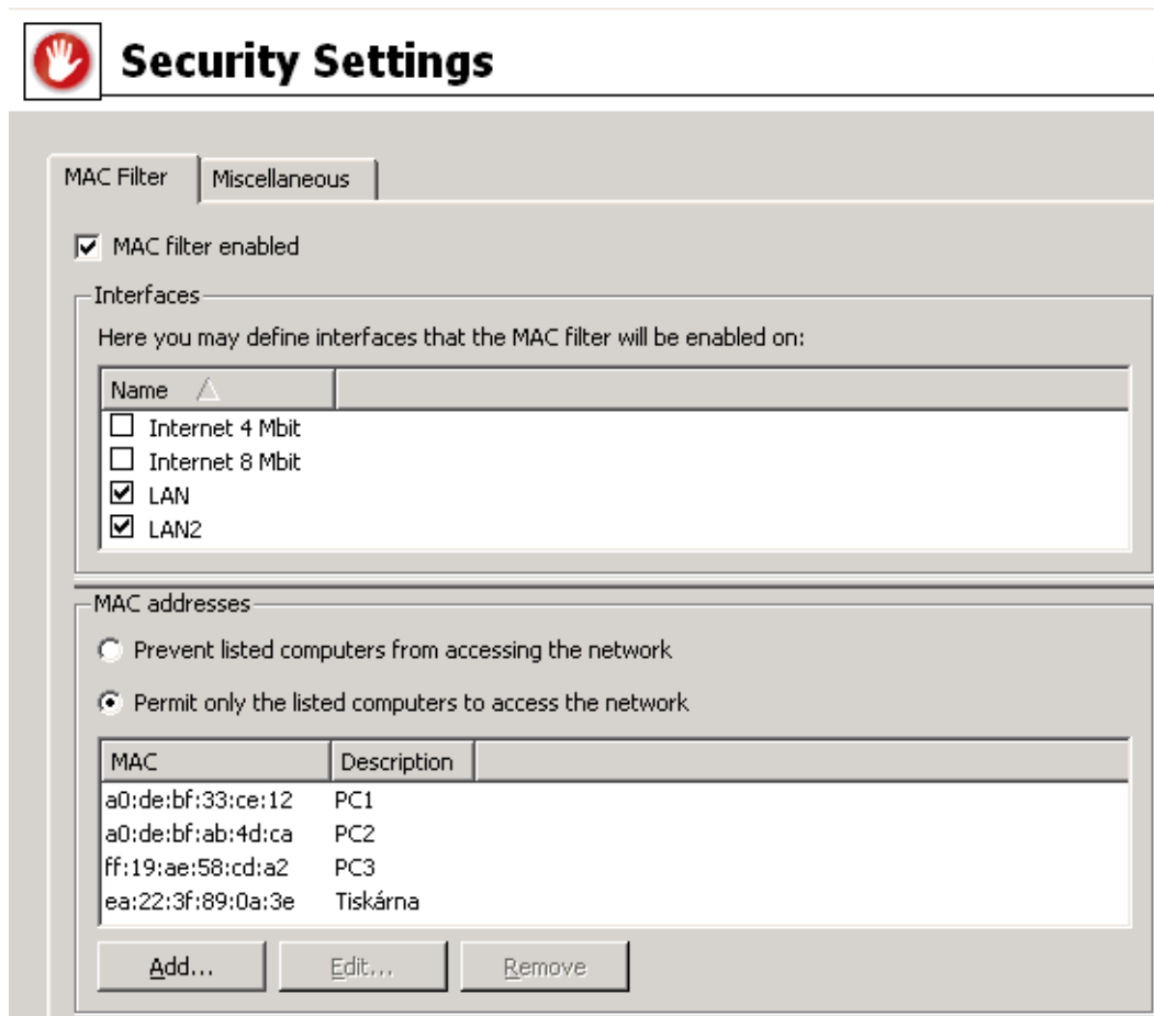
Figure 8.3 MAC address filtering
