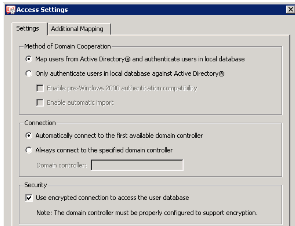
Figure 16.13 Advanced options for cooperation with the Active Directory.
