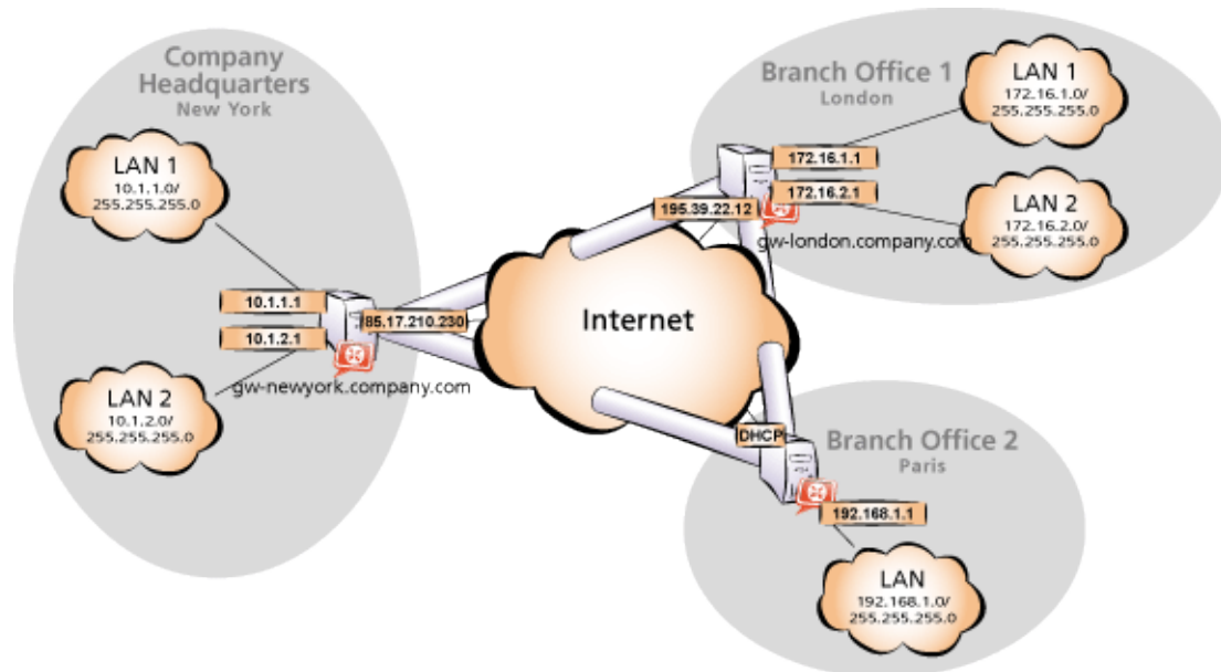
Figure 23.28 Example of a VPN configuration — a company with two filials
