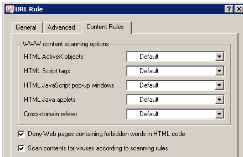
Figure 13.10 A rule filtering web pages by word occurrence (word filtering)
