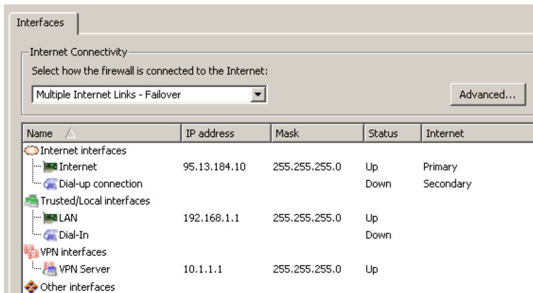
Figure 6.9 Configuration of interfaces — Internet connection failover
