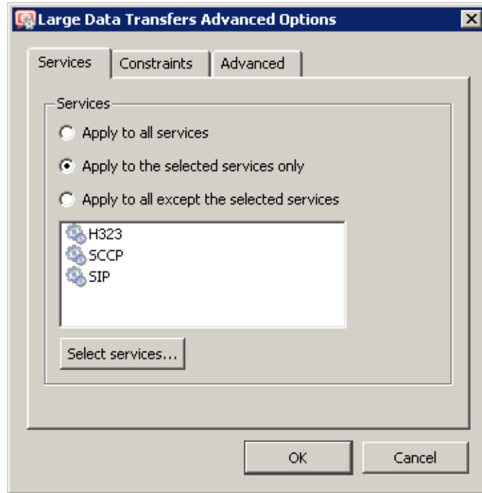
Figure 10.2 Bandwidth Limiter — network services
