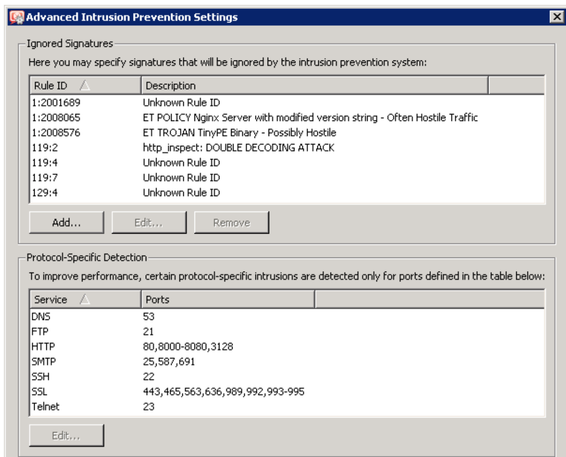
Figure 8.2 Intrusion prevention system advanced options
