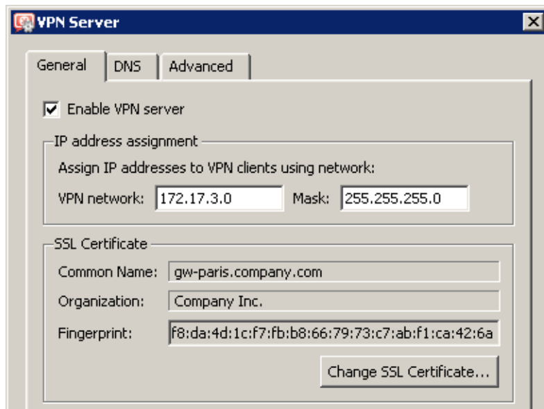
Figure 23.50 The Paris filial office — VPN server configuration
