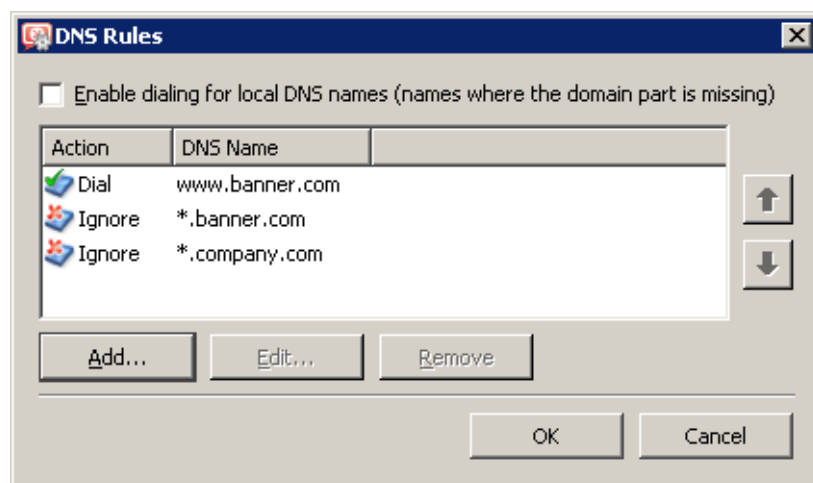
Figure 25.5 Dial on demand rules (for dialing based on DNS queries)
