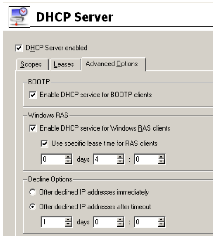
Figure 9.13 DHCP server — advanced options
