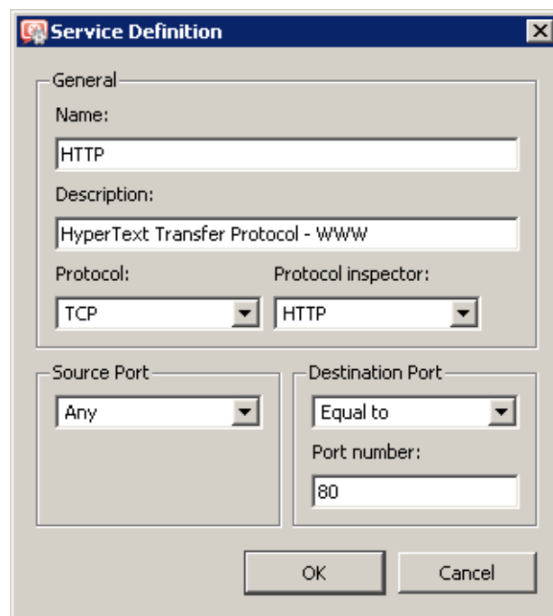
Figure 15.6 Network service definition
