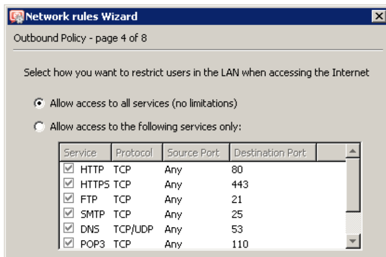
Figure 23.29 Headquarters — no restrictions are applied to accessing the Internet from the LAN
