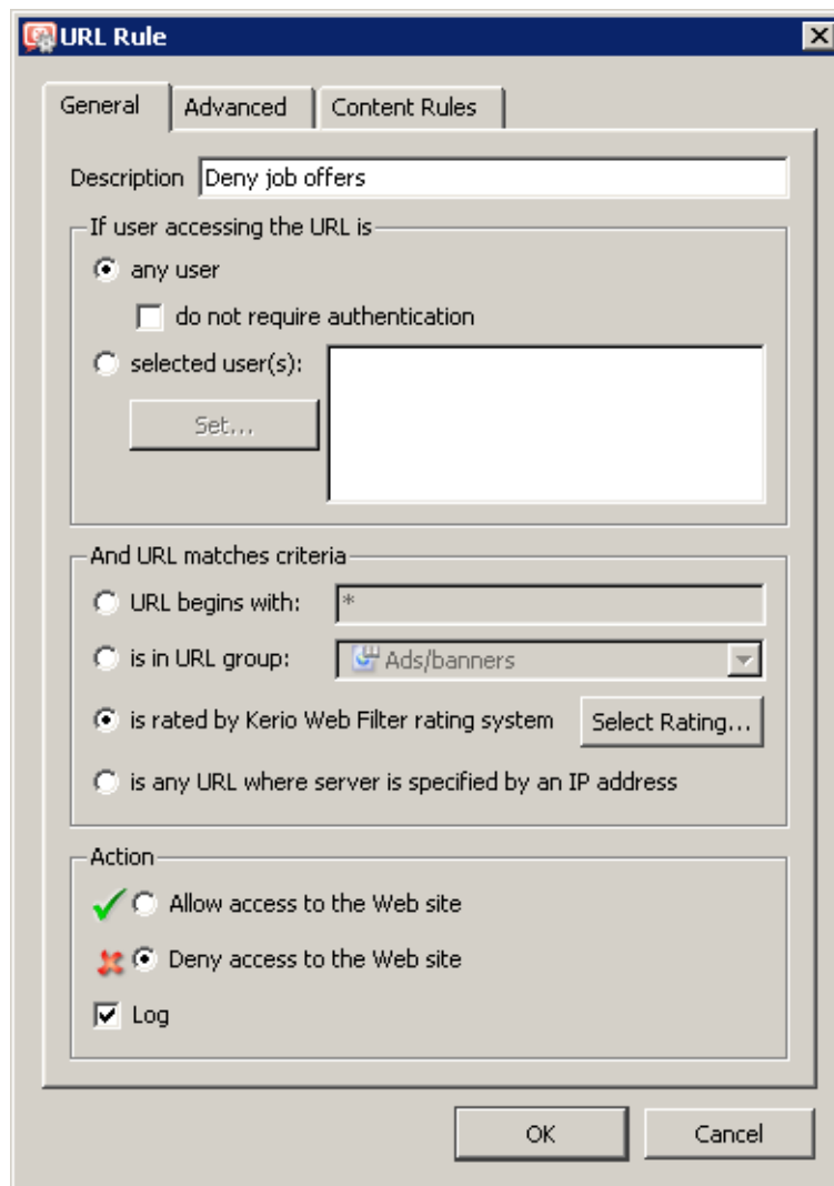
Figure 13.7 Kerio Web Filter rule
