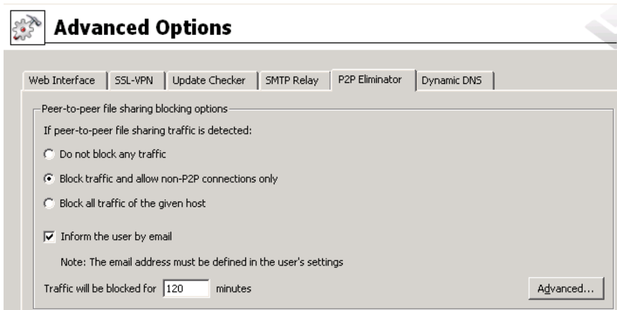
Figure 8.5 Detection settings and P2P Eliminator
