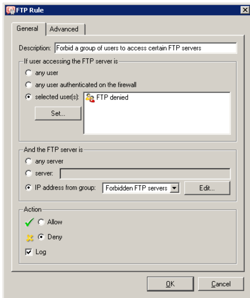
Figure 13.14 FTP Rule — basic parameters
