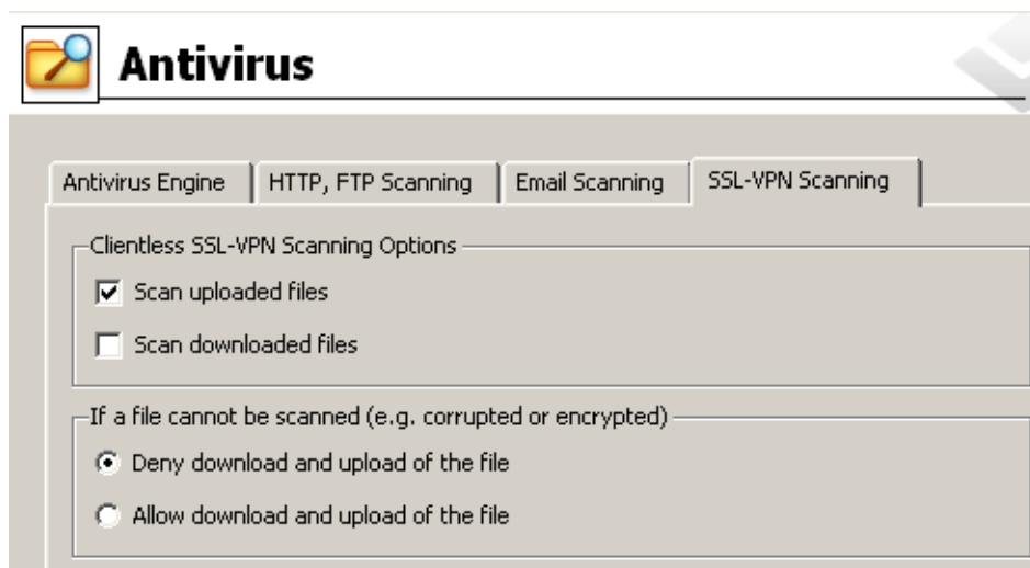
Figure 14.10 Settings for scanning of files transferred via Clientless SSL-VPN
