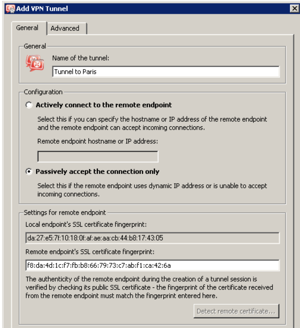
Figure 23.36 The headquarters — definition of VPN tunnel for the Paris filial
