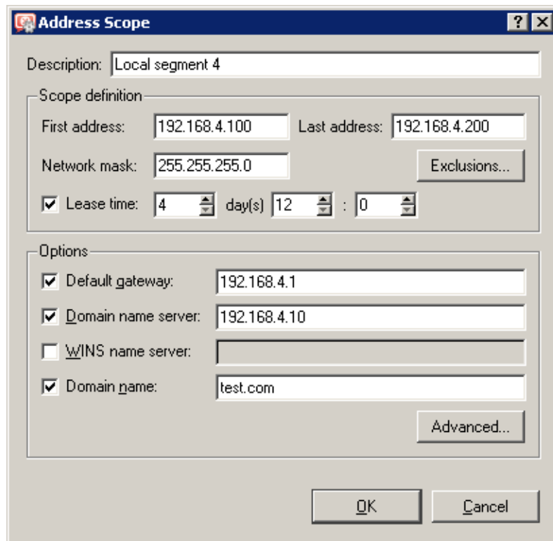
Figure 9.7 DHCP server — IP scopes definition
