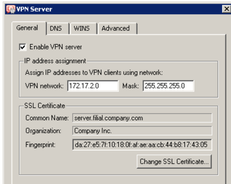
Figure 23.25 Filial office — VPN server configuration
