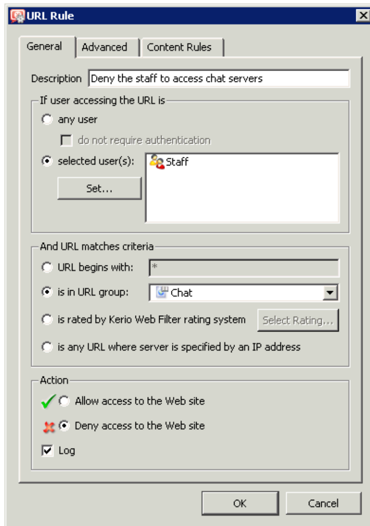
Figure 13.2 URL Rule — basic parameters
