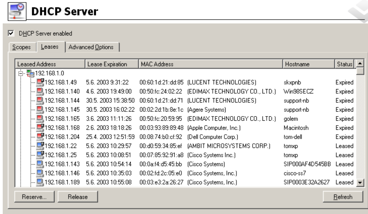
Figure 9.12 DHCP server — list of leased and reserved IP addresses
