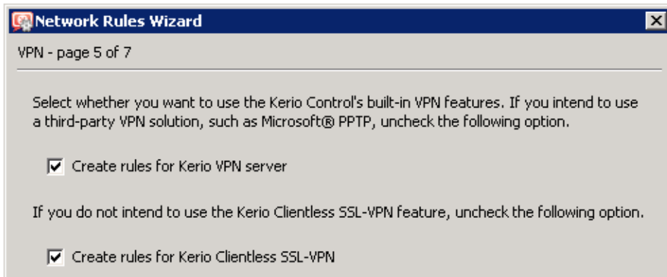
Figure 23.30 Headquarter — creating default traffic rules for Kerio VPN
