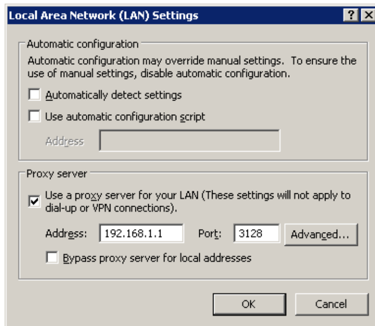
Figure 25.3 Configuring proxy server in Internet Explorer
