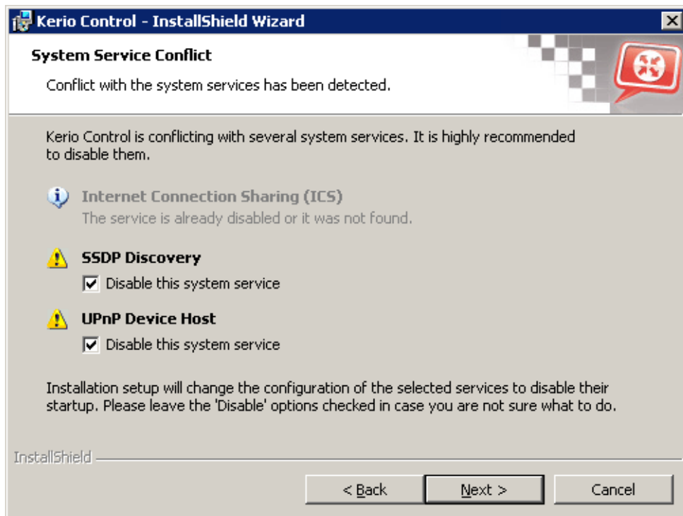
Figure 2.2 Disabling colliding system services during installation
