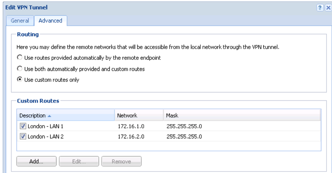
Figure 25.16 The headquarters — routing configuration for the tunnel connected to the London filial
