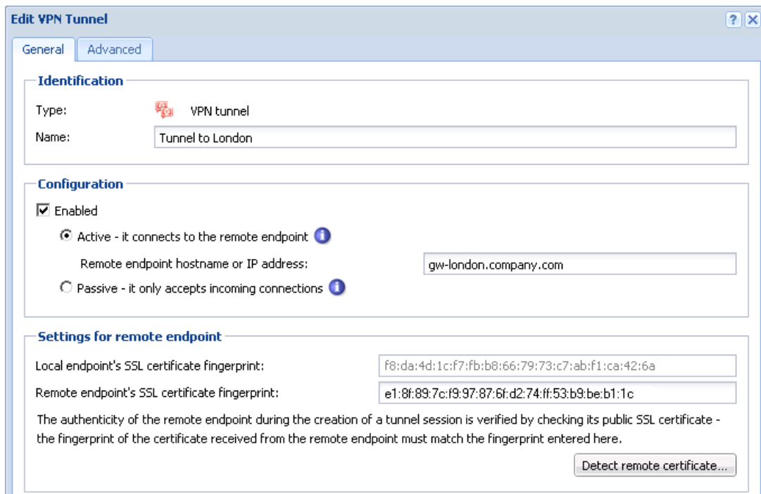
Figure 25.28 The Paris filial office — definition of VPN tunnel for the London filial office
