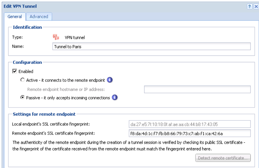
Figure 25.17 The headquarters — definition of VPN tunnel for the Paris filial
