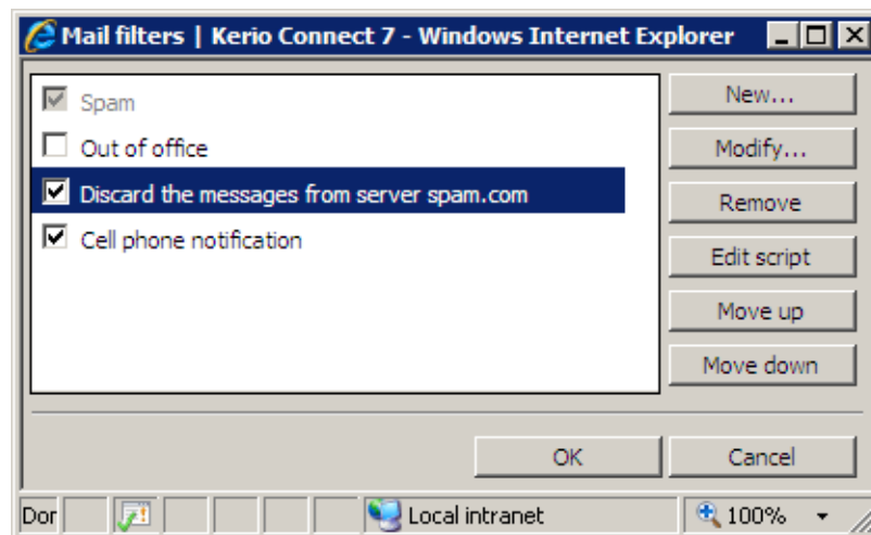
Figure 1.103 Rule list
