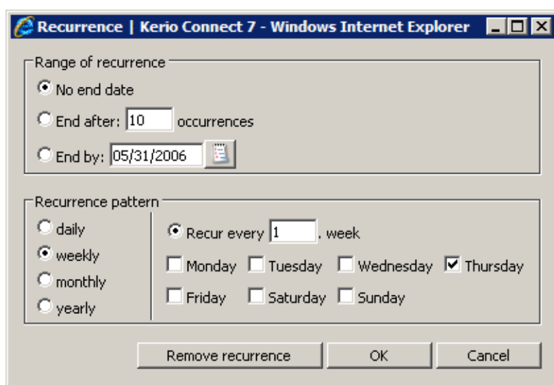
Figure 1.52 Event recurrence
