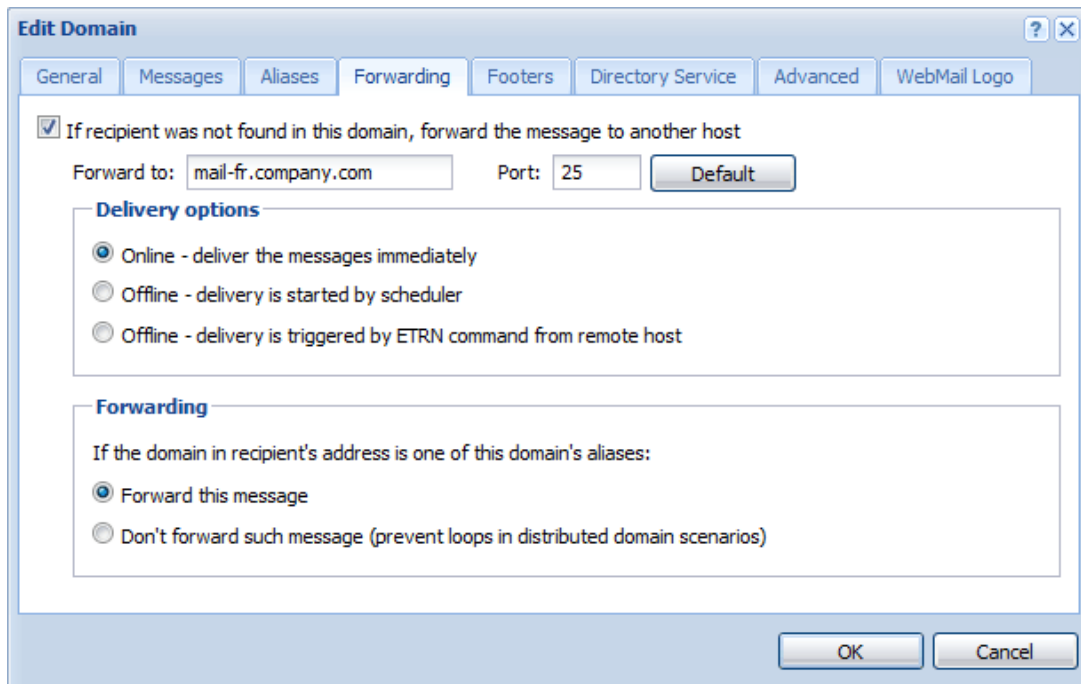
Figure 7.12 Forwarding settings
