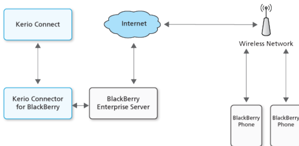
Figure 38.1 Kerio Connector for BlackBerry implementation example
