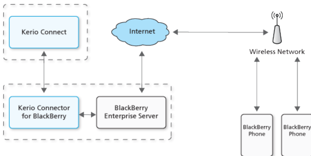
Figure 38.2 Installation on two separate computers
