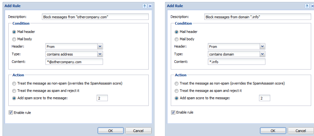
Figure 13.7 Rule definition — using wildcard
