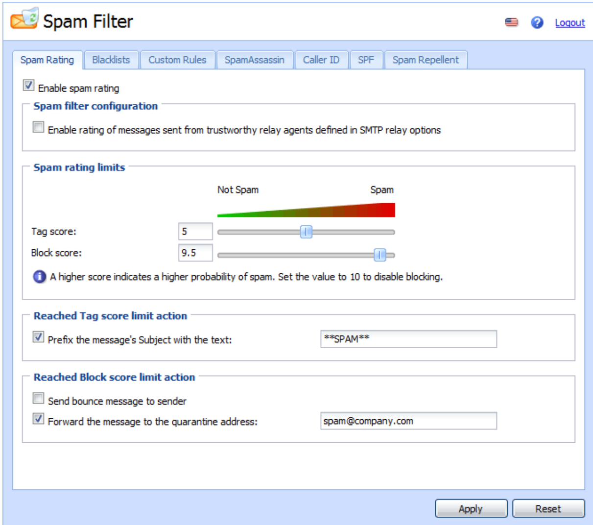
Figure 13.1 Spam Rating tab
