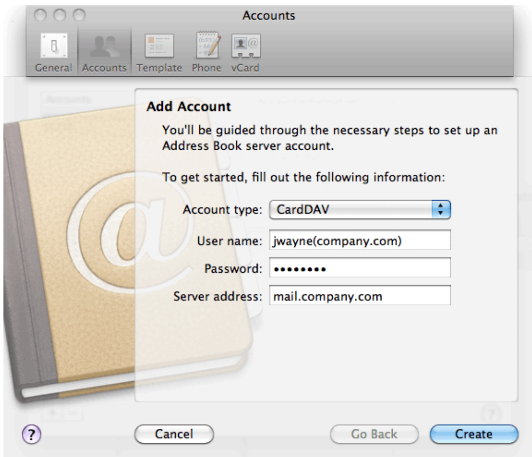
Figure 35.1 CardDAV account settings
