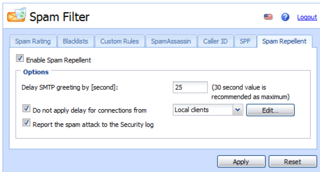
Figure 13.10 Spam repellent
