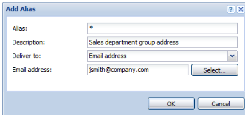
Figure 12.6 Defining Alias
