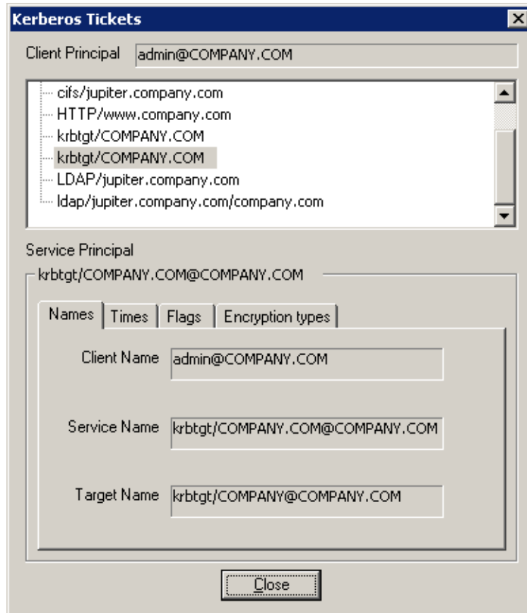
Figure 26.2 Kerberos tickets displayed in Kerbtray
