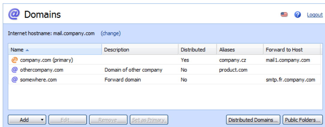
Figure 11.2 List of domains with a distributed domain
