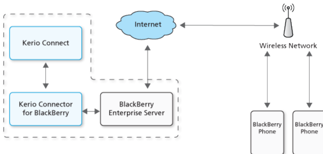
Figure 38.3 Installation on a single computer
