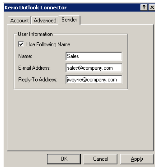
Figure 31.12 Account settings — sender information settings
