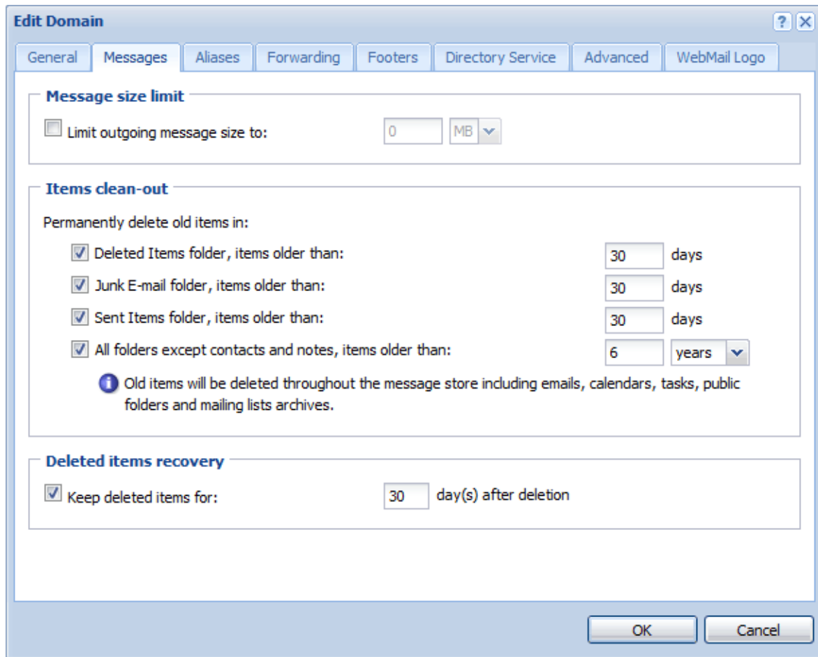
Figure 7.5 Domain Settings — Messages
