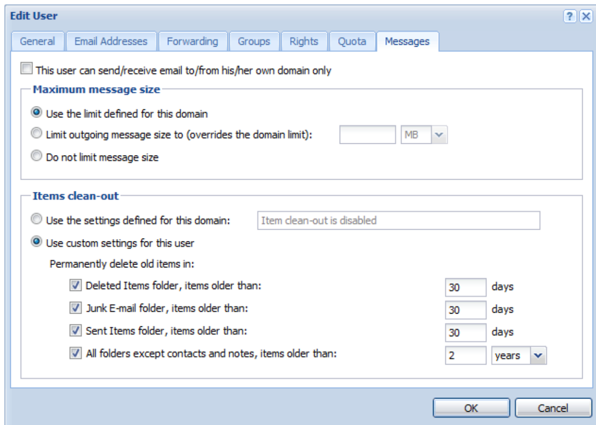
Figure 7.6 Setting of automatic clear-out for particular users
