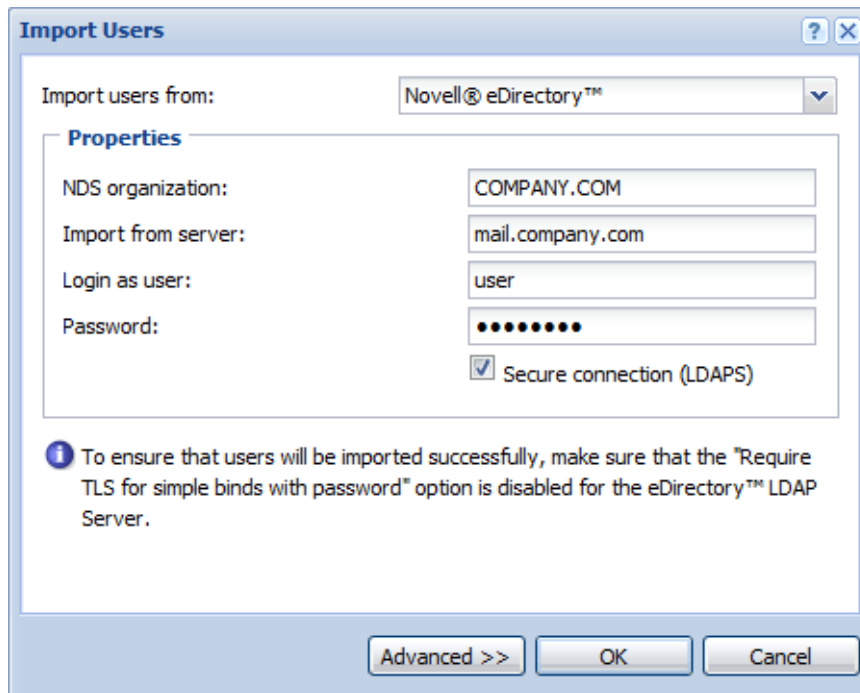
Figure 8.20 Import users from Novell eDirectory
