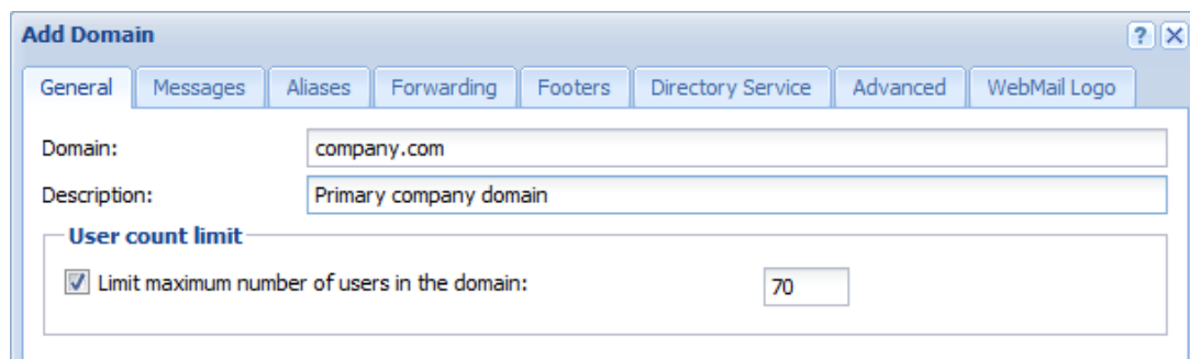
Figure 7.3 Domain settings — basic parameters
