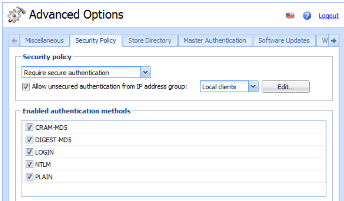
Figure 12.19 Security Policy tab
