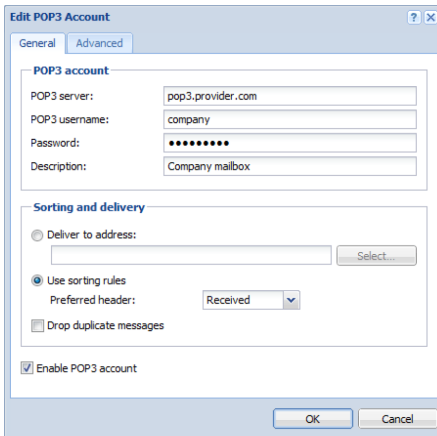
Figure 12.9 Defining Remote Mailboxes
