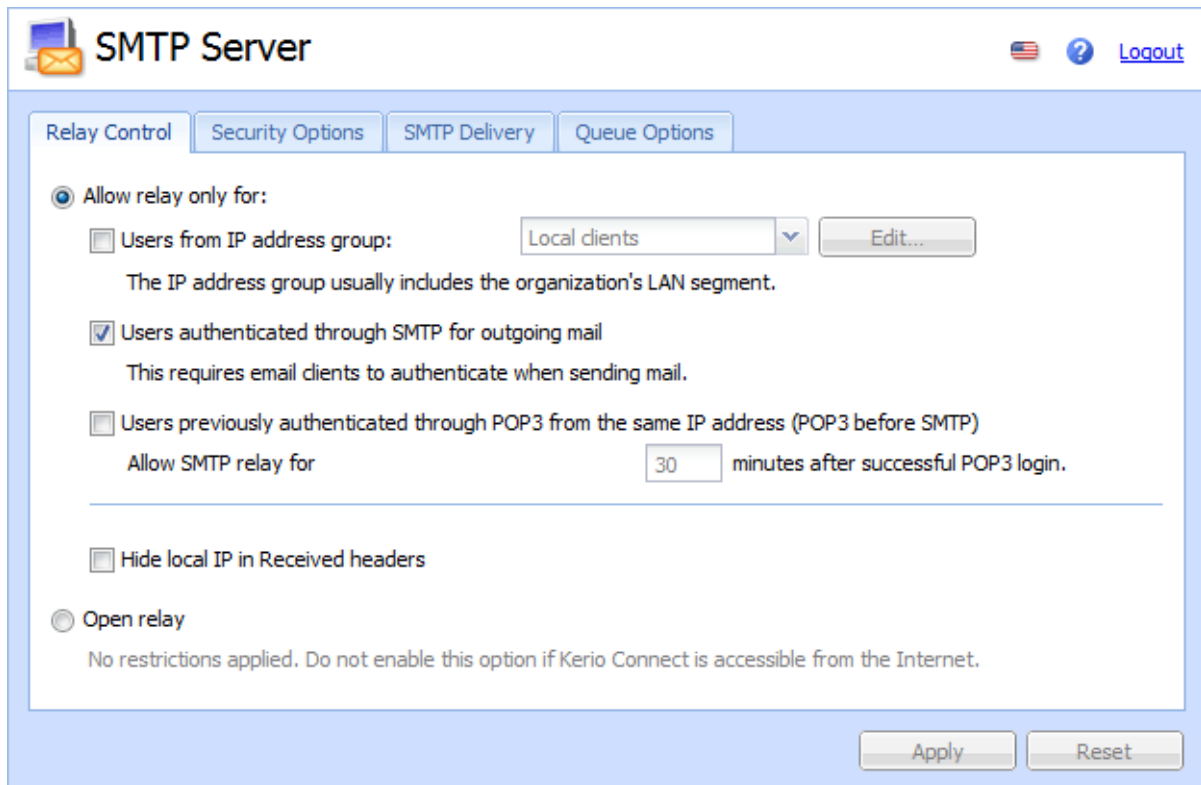
Figure 12.1 Relay Control tab
