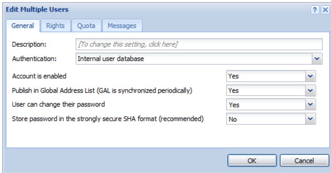
Figure 8.12 Bulk change of user accounts
